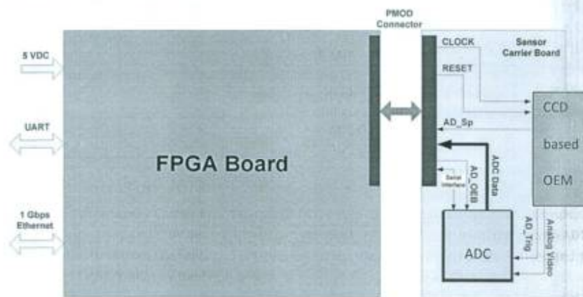
Figure 1. Interface Board: Functional Block Diagram
