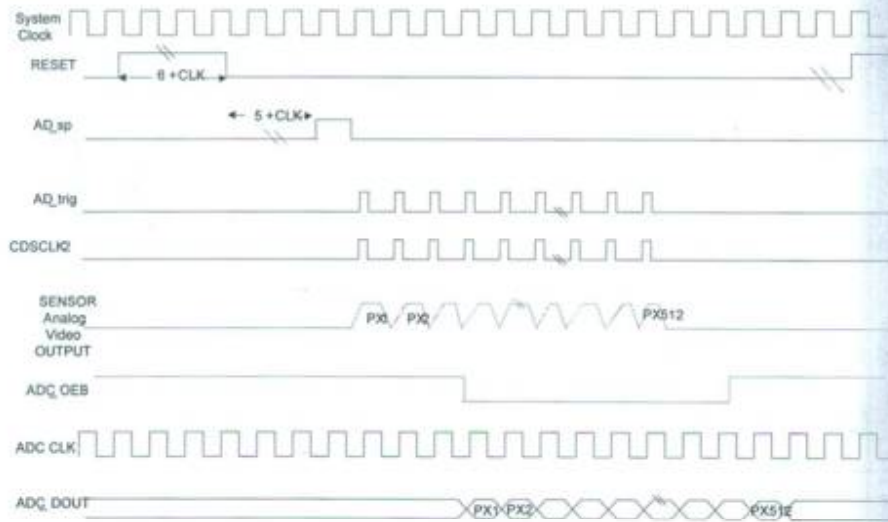
Figure 2: Timing Diagram
