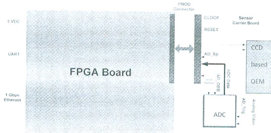
Figure 1 Interface Board: Functional Block Diagram
